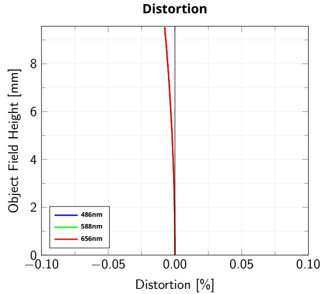
Object Field Height vs. Distortion, from the optical axis to the corner of the field of view
